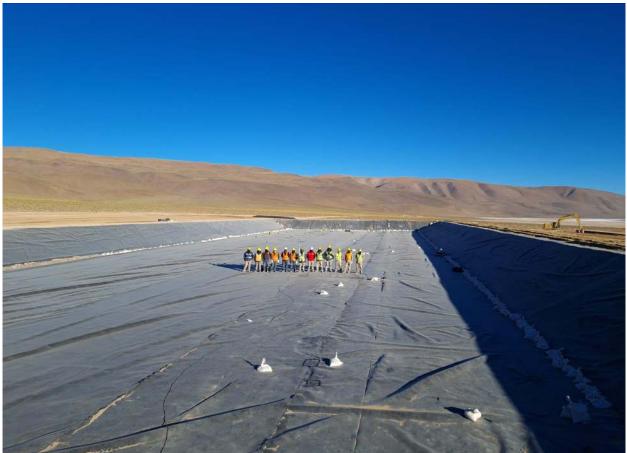
Figure 3: Evaporation Pond S1 Construction
