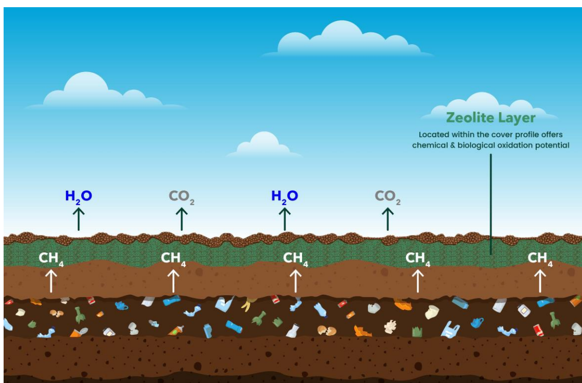
A layer of manufactured zeolite (indicated in green above) located within the cover profile offers the potential for chemical and biological oxidation.
